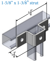
9051UF 3-hole "u" support for 1-5/8" x 1-3/8" strut
